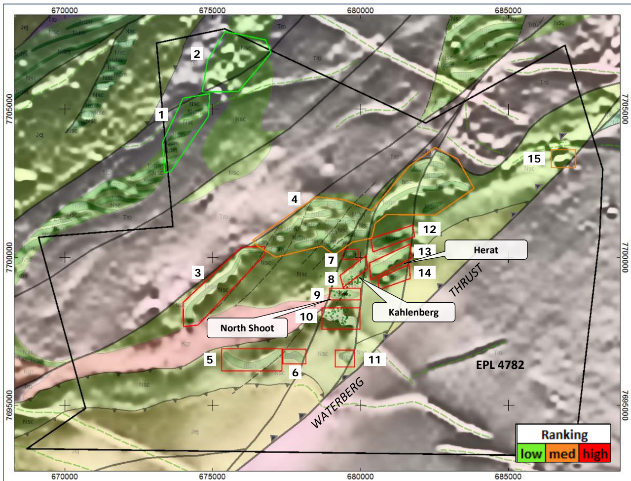
Figure 1: Joubira Zinc Project targets areas identified in the Terra Resources report with aeromagnetic interpretation shown over First Vertical Derivative Reduced to Pole (1VD RTP) aeromagnetic image
