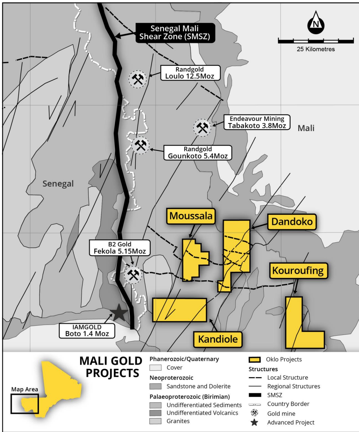
Figure 1: Location of the Dandoko, Moussala, Kouroufing and Kandiole gold projects in west Mali.
