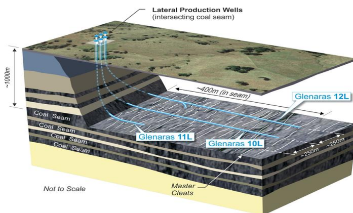
Figure 1 – Glenaras multi-lateral pilot
