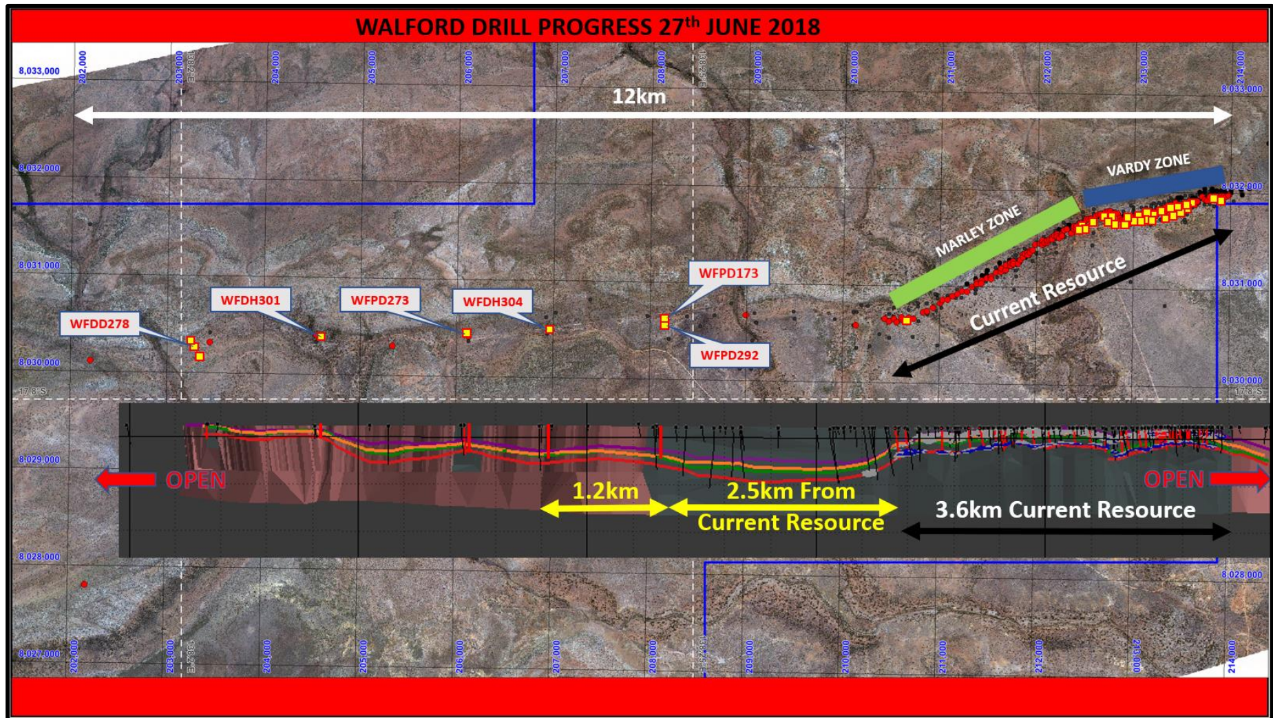
Figure 3 Location of completed holes including current extended hole WFPD173 and hole WFPD292 where results are awaited along strike from the Resource. The plan shows indicative planned holes (red) and the location of the prospective stratigraphy in the Long Section
