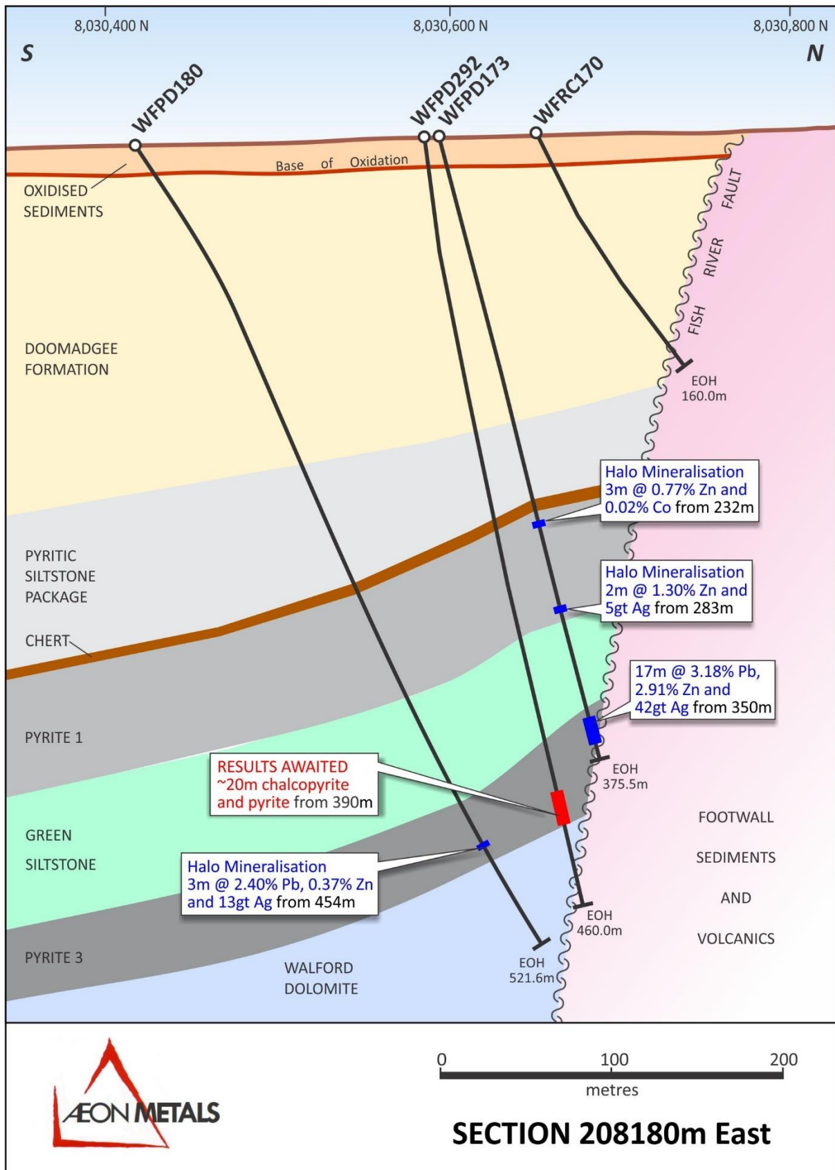
Figure 2 Section 208180E Geological section showing current hole WFPD173 and WFPD292
