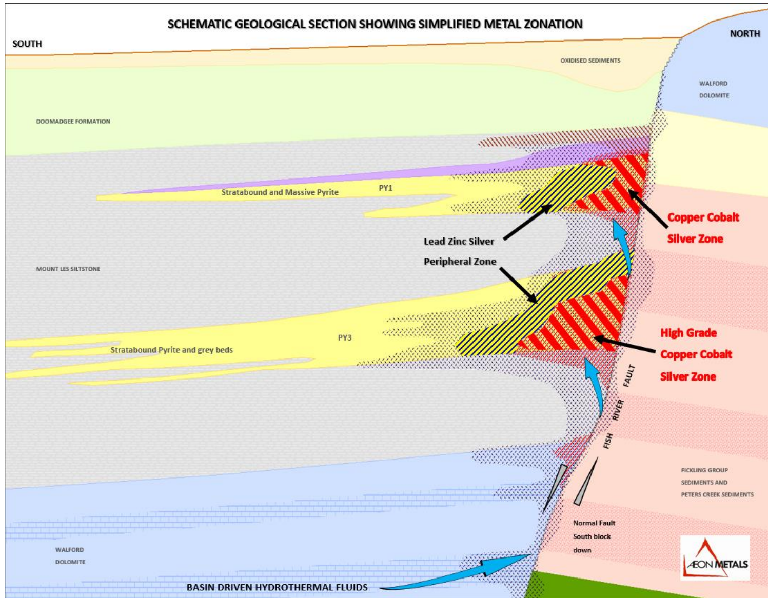
Figure 4 Schematic geological section showing zonation of mineralisation including Peripheral Zone mineralisation as intersected in hole WFPD173
