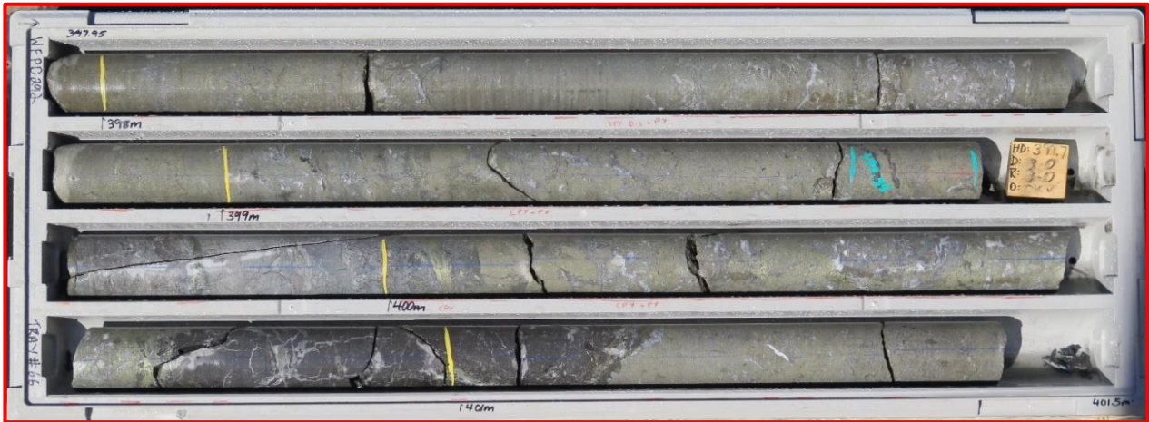
Figure 1 WFPD292 Tray 66 showing chalcopyrite overprinting massive to semi-massive sulphides within the Py3.
