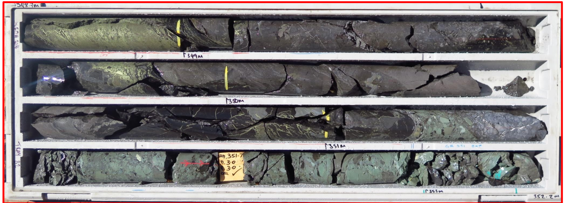
Figure 2: Tray 81 from hole WFDH304 showing typical high grade massive chalcopyrite and zones of fracture fill chalcopyrite in shale units. The zone consisted of approximately 19m intersection of chalcopyrite with pyrite and minor galena and sphalerite.
