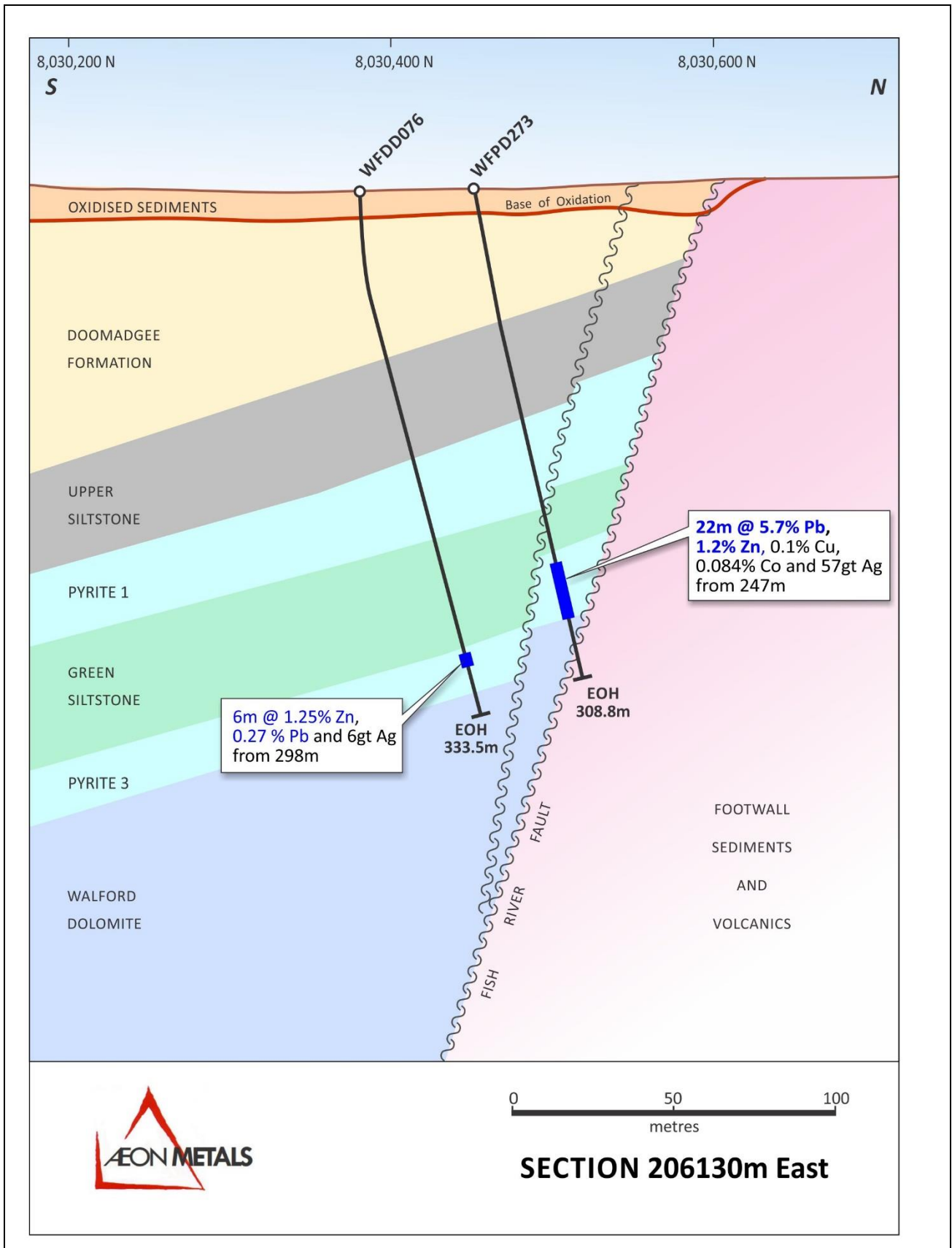
Figure 3: Section for hole WFPD273 showing secondary fault sub-parallel to the Fish River fault with upthrown block of high grade base metal mineralisation offset from weak low grade zinc and lead mineralisation seen in old WMC hole WFDD76. Grid squares are 200m.
