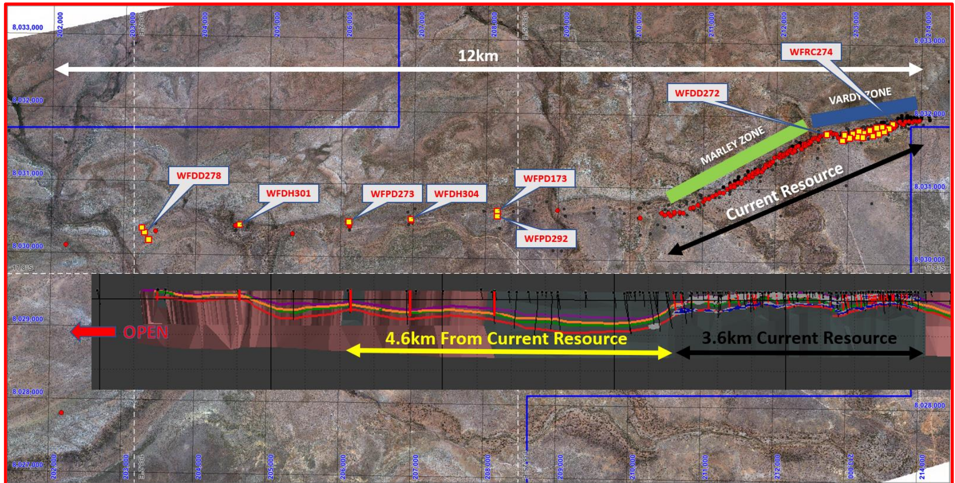
Figure 1: General location plan showing hole WFPD273, 4.6 kilometres west of the current resource. Previously reported holes WFDD272 and WFRC274 shown inside Vardy Resource. Other completed holes are shown in yellow, indicative planned holes as red dots and the currently interpreted prospective stratigraphy in long section view.
